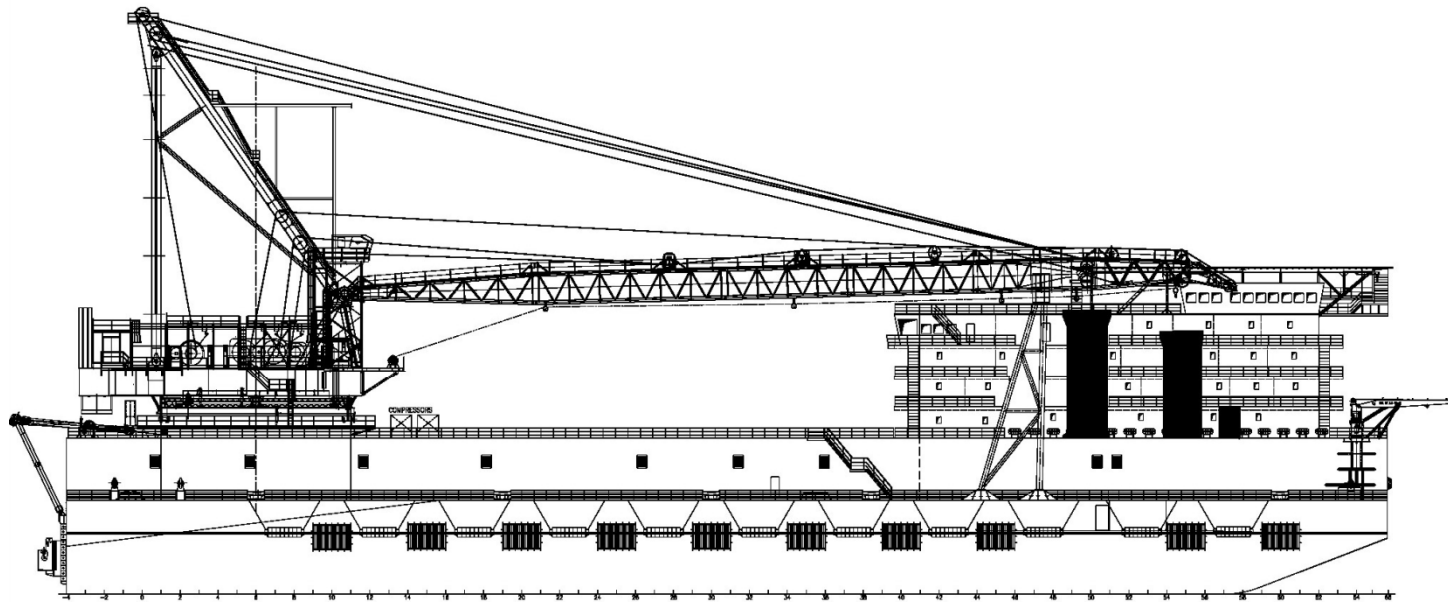
PROFILE VIEW
